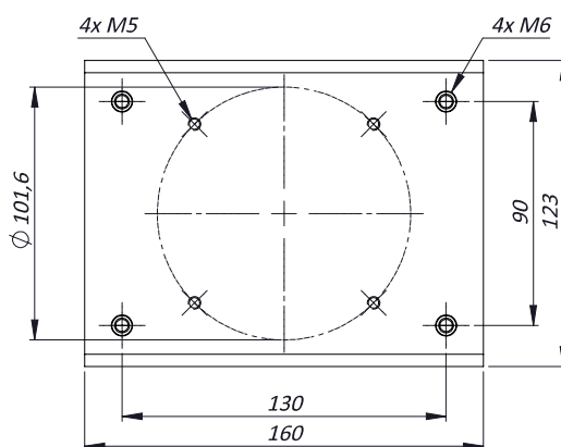
MOUNTING PATTERN
