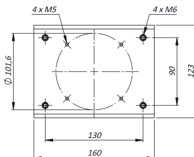
MOUNTING PATTERN
