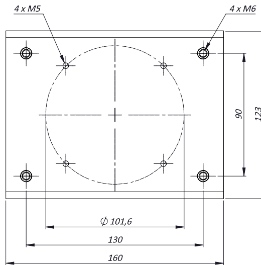
MOUNTING PATTERN
