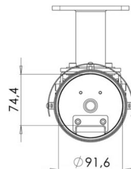
FRONTAL VIEW
