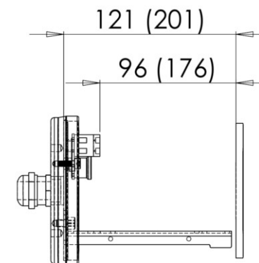
Internal dimensions
